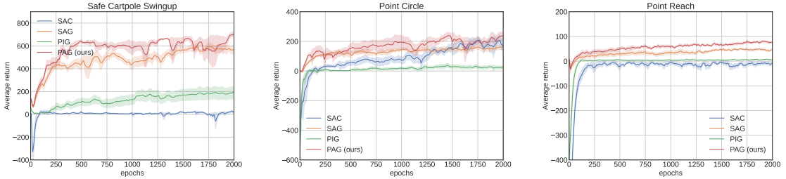
Figure 6: Overall performances comparing PAG with SAC, SAG and PIG on 3 different environments with repulsive policies.
