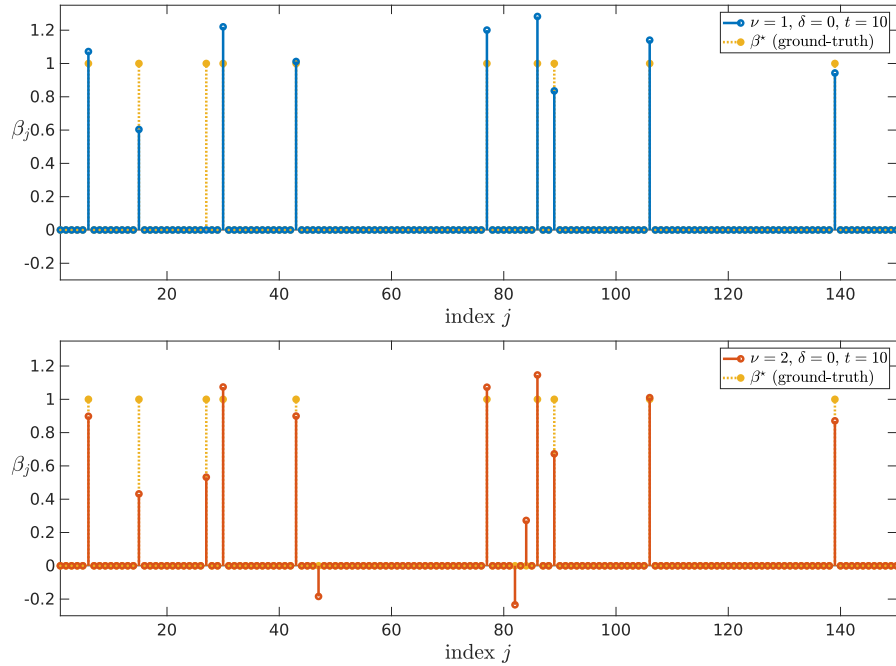
FIG 16. \ell^q constrained minimization in high dimension ( n = 300, p = 150 ). We used Algorithm 6 to process a synthetical dataset (X, \beta^*, y) with dimensions n = 300 and p = 150 . The ground-truth vector \beta^* is displayed above using yellow dotted stems. As can be seen above, \beta^* has ten nonzero entries ( \mathcal{L}_0(\beta^*) = 10 ) which encourages us to set t = 10 in problem (62). Thus, Algorithm 6 was run using t = 10, q = 0.7, \delta = 0 and \nu = 1 (top) or \nu = 2 (bottom). In this experiment, Algorithm 6 was initialized using a random initial guess \beta^{(0)} lying in the constraint set \mathcal{B}_q(t^{1/q}) . We can see that both settings of \nu yielded an output with \mathcal{L}_0 norm close to t = 10 (that is, nine for \nu = 1 and thirteen for \nu = 2 ). The setting \nu = 1 yields here slightly sparser output (blue plain stems) than that obtained using \nu = 2 (orange plain stems), which is a general observation that we also made on many other simulations. As mentioned above, this behavior is probably due to the sparsity-promoting diamond shapes (when \nu = 1 ) of the constraint sets in (69b). Besides, we could observe that convergence of the iterates was roughly fifteen times faster with \nu = 1 than with \nu = 2 on this dataset. More generally significantly faster convergence was achieved with \nu = 1 than with \nu = 2 in all our the experiments that we made.
