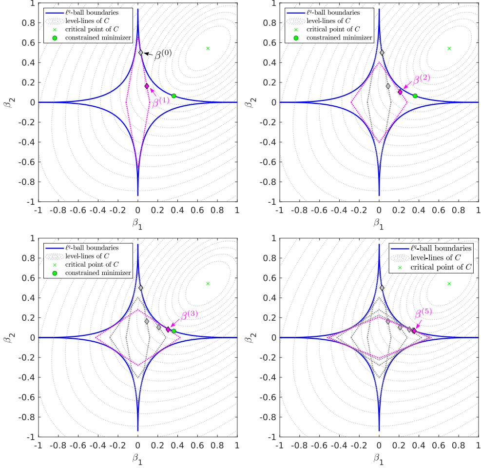
Fig. 13 \ell^q constrained minimization using Algorithm 5 with \nu = 1 ). We display (with the same displaying rules as in Fig.12) the first five iterates generated by Algorithm 5 with \nu = 1 applied to the same dataset as that considered in Fig. 12. While in Fig. 12 the setting \nu = 2 yielded ellipsoid shaped constraint sets \mathcal{E}_q^\nu(\eta^{(k+1)}, t) , the setting \nu = 1 yields diamond shaped constraint sets. We can see that, as in Fig. 12, the numerical scheme seems to successfully converge toward the solution of (63) (green disk). We can also notice that, over this dataset, the setting \nu = 1 yields a faster convergence than the setting \nu = 2 (see Fig. 12). Our experiments in larger dimensions (not shown here) tend to confirm that \nu = 1 yields a significantly higher convergence rate than the setting \nu = 2 .
