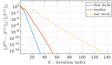
(b) Algorithm 3 with q = 0.1
