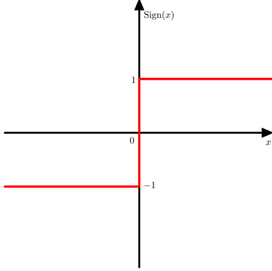
Figure 1: Sign function in \mathbb{R}
