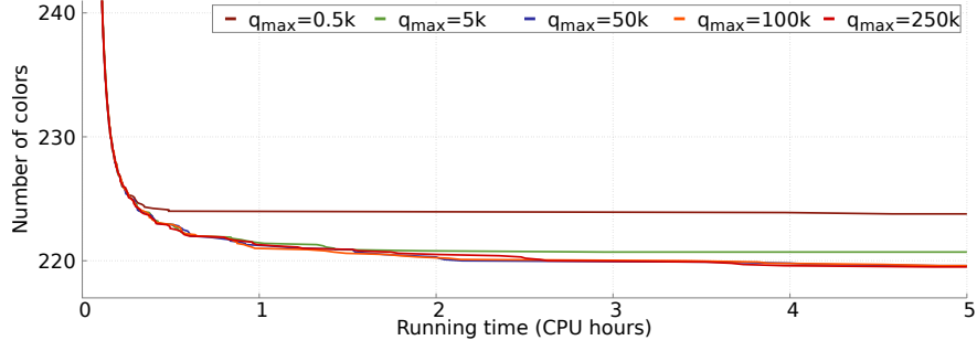
Fig. 3. Number of colors over time with different values of q_{\max} obtained on the instance vispecn13806. Parameters are \sigma = 0.15 , p = 1.2 , no clique knowledge, and no BDFS.
