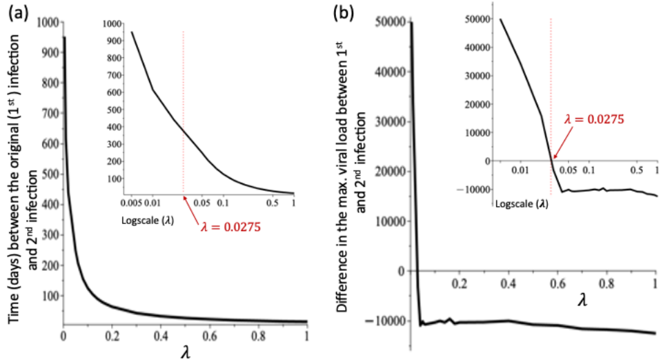
Figure 5: (a) Time between the 1 st and 2 nd viral infections, as we vary \lambda . (b) Difference in the maximum viral load during the 1 st and 2 nd viral infections: the threshold between positive values (i.e., 1 st wave higher than the 2 nd wave) and negative values (i.e., 1 st wave lower than the 2 nd wave) is at \lambda \approx 0.0275 . The inset sub-figures are the same as the main figures, but with the horizontal axis on a logscale. All other model parameters are as in Table 2.
