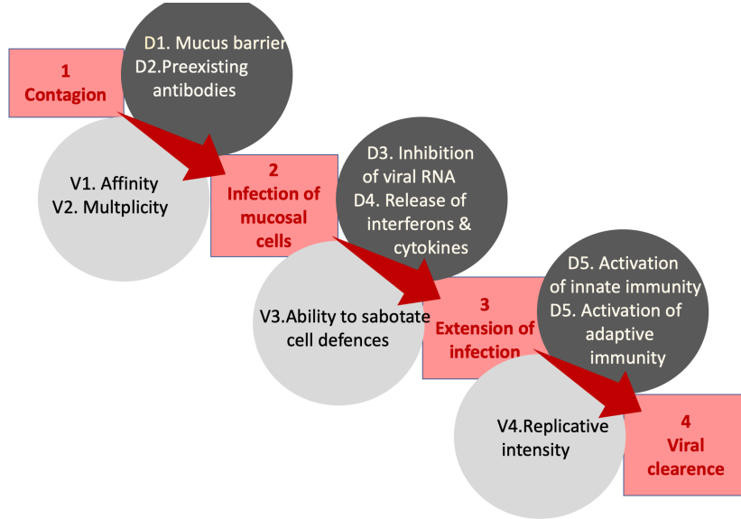
Figure 1: Representation of the in-host dynamics of the virus and of the immune response.
