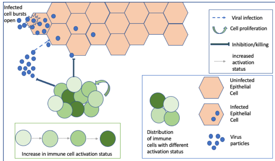
Figure 2: Caricature description of the variables that form the functional subsystems considered in this study. The virus particles and the infected epithelial cells are described by densities, while the immune cells are described by a distribution over the activity variable.
