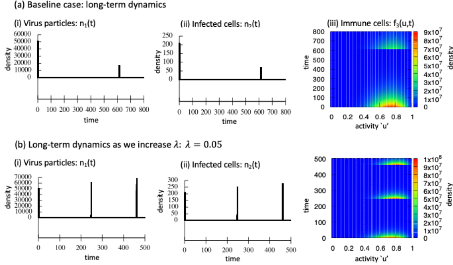
Figure 4: (a) Long-term baseline dynamics of model (10); the parameters are as in Figure 3. (b) Long-term dynamics obtained when we increase the death rate of immune cells to \lambda = 0.05 .; all other parameters are as in Table 2. In sub-panels we show: (i) 2D plot of the density of virus particles n_1(t) ; (ii) 2D plot of the density of infected cells; (iii) 3D plot of the distribution of immune cells f_3(u, t) . We see that for (a) the second infection is weaker than the first one, while for (b) the second infection is stronger than the first one.
