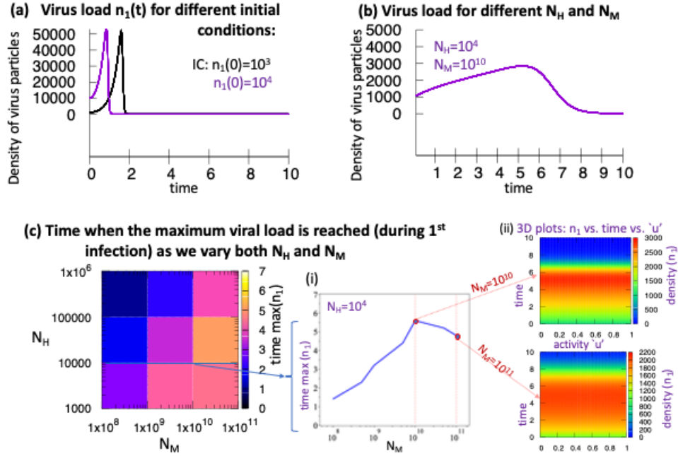
Figure 7: (a) Dynamics of n_1(t) when we increase the initial viral load: from n_1(0) = 10^3 to n_1(0) = 10^4 . All other parameters are as in Table 2. (b) Dynamics of n_1(t) when we decrease N_H (from baseline N_H = 10^5 ) and increase N_M (from baseline N_M = 10^9 ). For a more thorough investigation of the effect of varying N_H and N_M on viral load, in panel (c) we show a colormap of the time when n_1 reaches a maximum value, as we vary N_M \in [10^8, 10^{11}] and N_H \in [10^3, 10^6] . The inset sub-figures in panel (c) show: (i) a change in the time when n_1(t) reaches its maximum value for N_H = 10^4 and N_M \in [10^8, 10^{11}] ; (ii) the 3D plots of n_1(t) vs. time( t ) vs. activity ( u ) for 2 specific cases: N_M = 10^{10} (top) where \max(n_1) is reached at t \approx 5.5 but the virus is eliminated after t = 8 ; N_M = 10^{11} (bottom) where \max(n_1) is reached at t \approx 5 but the virus is eliminated after t = 9.5 .
