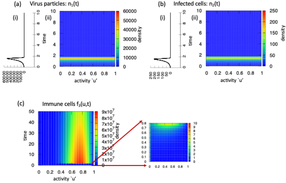
Figure 3: Baseline dynamics of continuum model (10). (a) density of virus particles: n_1(t) ; (b) density of infected cells: n_2(t) ; (c) distribution of immune cells across the activity space: f_3(t, u) . All parameters are as in Table 2. In (a),(b), the sub-panels (i) show the 2D plots n_{1,2}(t) vs. time, while the sub-panels (ii) show the 3D plots n_{1,2} vs. u vs. time. The inset (right) sub-figure in (c) shows the same graph as in the left main figure, but for time t \in [0, 0.8] , so that we see more clearly how the immune cells start to become activated (i.e., larger f_3(u, t) as u \rightarrow 1 and t \rightarrow 0.8 ).
