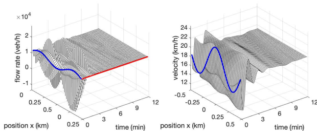
Fig. 3. Closed-loop simulation of traffic flow rate and velocity with the nominal control law (11) for a realization of the stochastic parameter \gamma(t) . The controlled flow rate evolution is highlighted in red.
