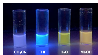
Fig. 4. Emission colours of 4a in various solvents after excitation at 365 nm (with [\mathbf{4a}] = 10^{-4} \text{ mol}\cdot\text{L}^{-1} ).
