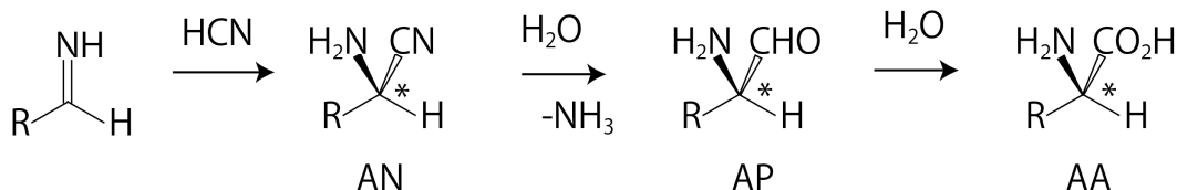
Fig. 1 Chiral intermediates leading to the formation of amino acid according to the Strecker synthesis. The precursors before L -amino acid (AA) are amino propanal (AP) and amino nitrile (AN).
