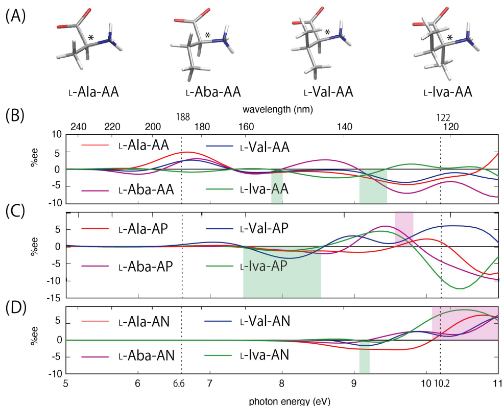
Fig. 2 (A) The most stable structures of L-amino acids: alanine (Ala), 2-aminobutyric acid (Aba), valine (Val) and isovaline (Iva) in zwitterion. The asterisks (*) indicate the chiral centers. AA
