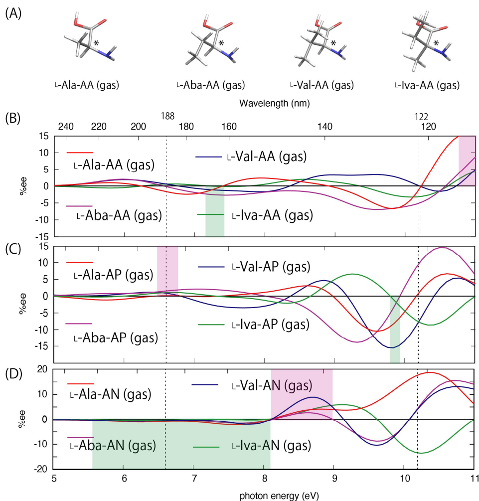
Fig. 3 (A) Most stable structures of L-Ala, L-Aba, L-Val and L-Iva in amino acid (AA) forms in gas phase. (B)-(D) Induced enantiomeric excess (%ee) of L-form chiral molecules by R-CPL in the
