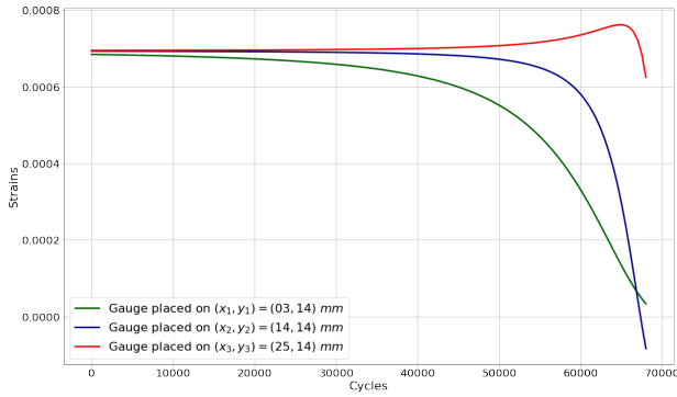
Fig. 4. Strain values time series corresponding to a sensor sample generated. In this illustration, three strain gauges are placed at the following positions (x, y) : (3, 14) , (14, 14) and (25, 14) mm.
