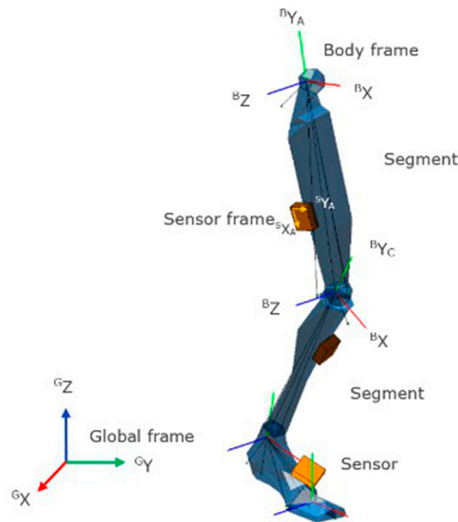
Figure 2. Xsens sensor reference frames and segment reference frames [40].
