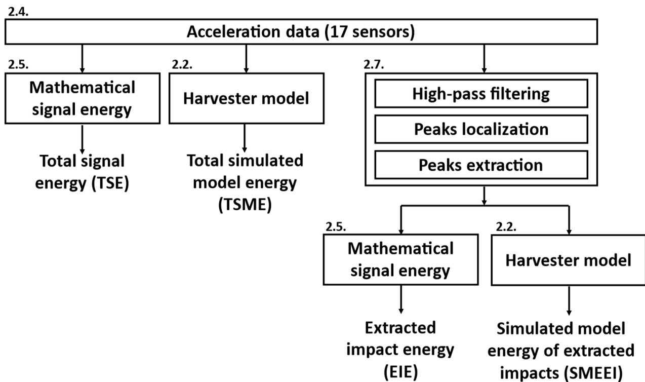
Figure 4. Flowchart of impact evaluation. The first step consists of calculating the mathematical signal energy and simulating the harvester model energy, using the total acceleration data. The second step consists of extracting the impacts from the acceleration data, and then calculating the new mathematical signal energy and simulating the new harvester model energy. The numbers displayed above the blocks represent the paper sections where the method is discussed.
