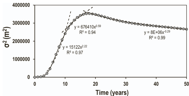
Fig. 18. Model estimates of the variance of sediment displacements.
