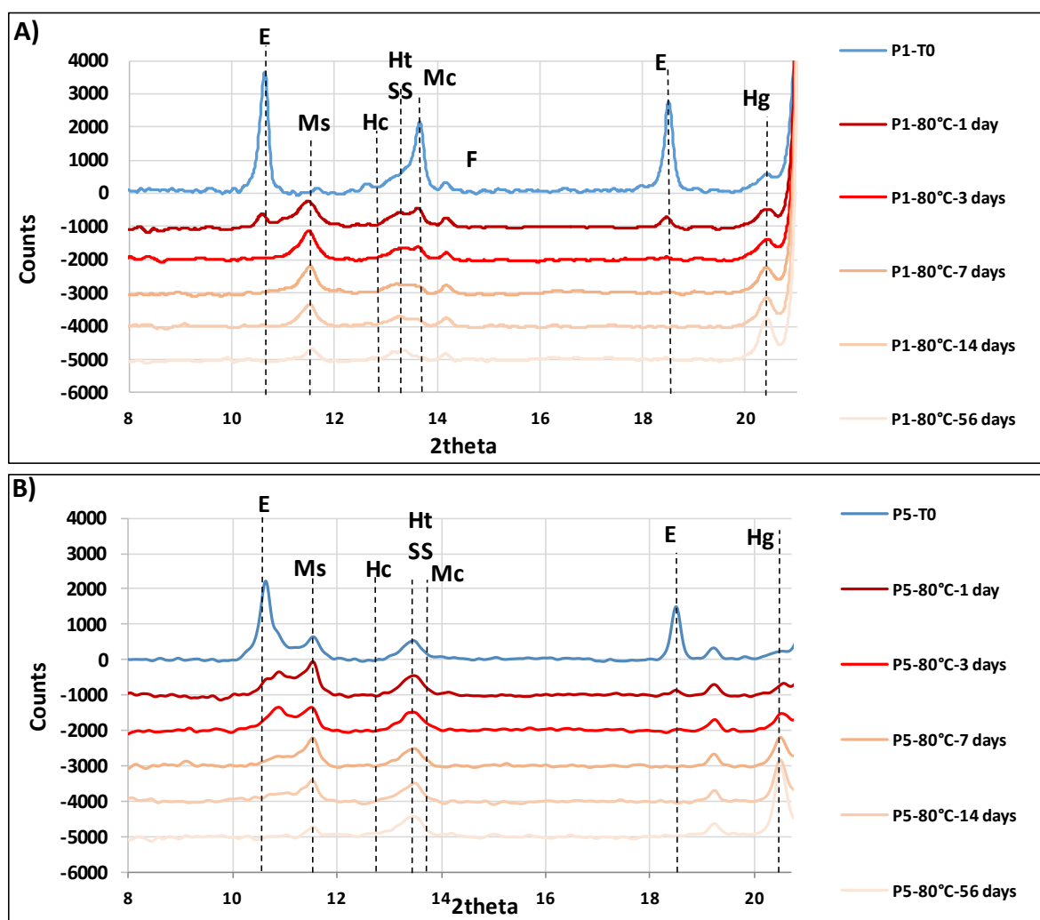
Figure B.1. Comparison of the partial XRD patterns as function of the TT of samples P1 and P5. E=Ettringite, Ms=Monosulfoaluminate, Hc=Hemicarboaluminate, Mc=Monocarboaluminate, F=C 4 AF, SS= solid solution, Ht=hydrotalcite et Hg=Hydrogarnet.
