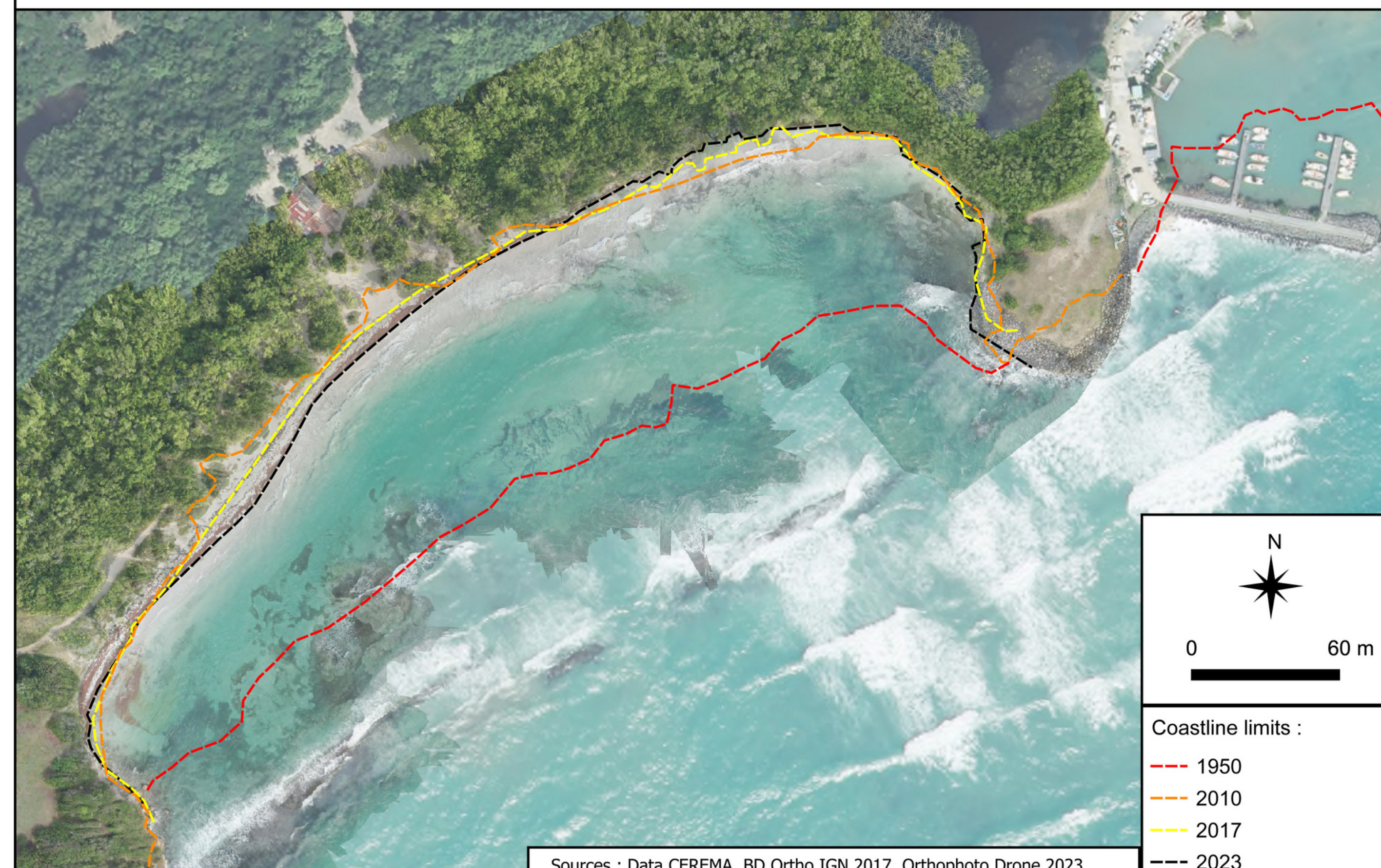
EVOLUTION OF COASTLINE FROM 1950 TO 2023 BEACH OF L'ANSE DUMONT (SAINT-FÉLIX, LE GOSIER, GUADELOUPE)
