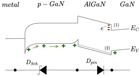
Fig. 1. Simplified band diagram of the gate stack of the DUT, the mechanism (1) is electron trapping at the interface AlGaIn/GaN, (2) is the hole depletion over the barrier to reach the buffer.
