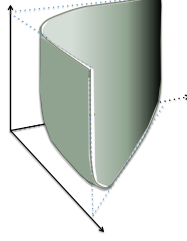
Figure 1: A smoothed corner of Q^\delta
