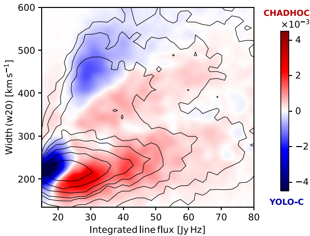
Figure 5. Team Minerva: Difference in the number of sources found between CHADHOC and YOLO-C catalogues in a flux against line width parameter space. The color encodes the difference in the local number of sources as a proportion of the total merged catalogue size (32652 predicted sources). The contours are the local number of sources averaged between the two catalogues with values: 6, 14, 30, 50, 64, 92, 128, 192. The density heatmap is computed on a 30 \times 30 grid and plotted with interpolation.
