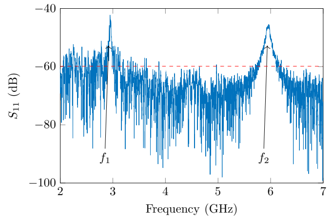
Fig. 19. Measured S-parameters with the empty measurement for a value of \phi = 70^\circ and \theta = 90^\circ in the office for a distance resonator-antenna of 20 cm. An averaging of 5 samples is used.
