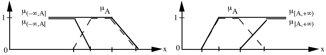
Figure 2: (a) points possibly/necessarily before A ; (b) points possibly/necessarily after A
