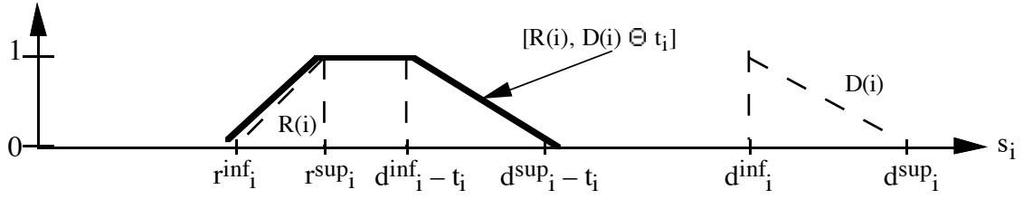
Figure 3: possible values for s_i given the temporal constraints on operation i .
