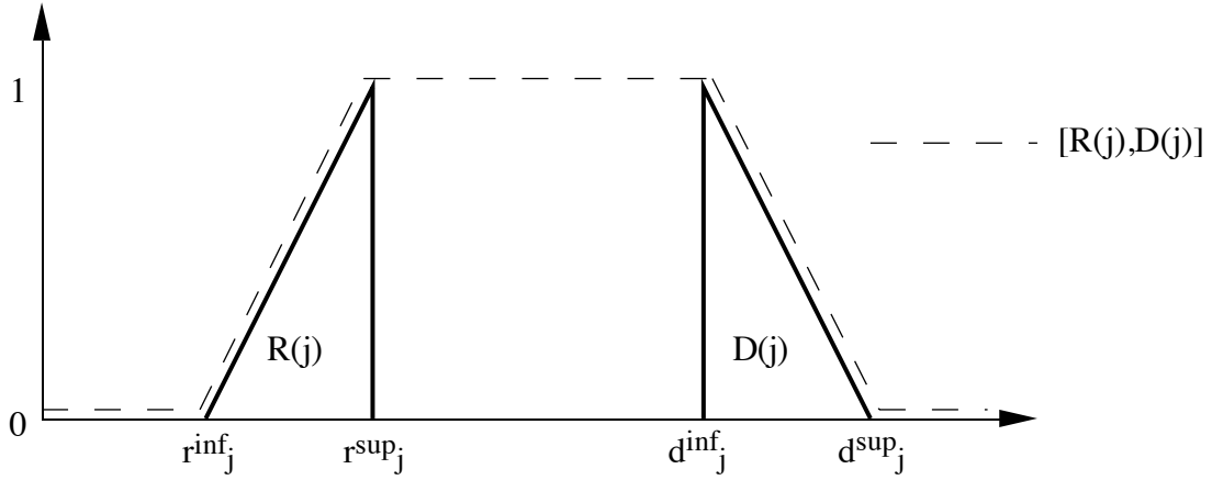
Figure 1: Fuzzy time horizon for job j
