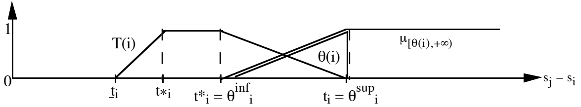
Figure 4: from [T(i), +\infty) to [\theta(i), +\infty)
