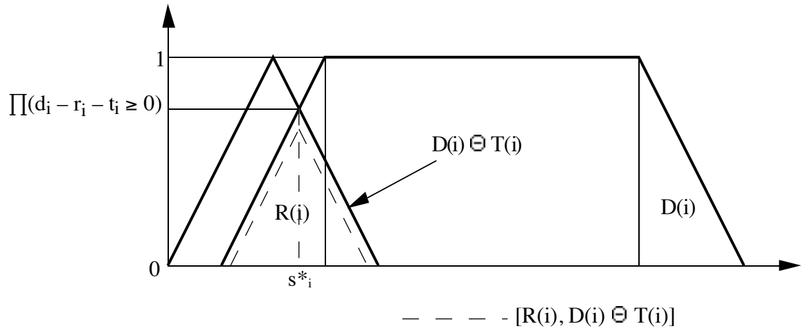
Figure 5: consistency degree of O_i 's temporal window
