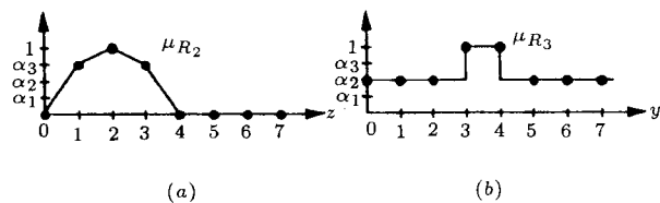
Figure 3. Modeling of C_2 (a) and C_3 (b) by means of fuzzy unary restriction.
