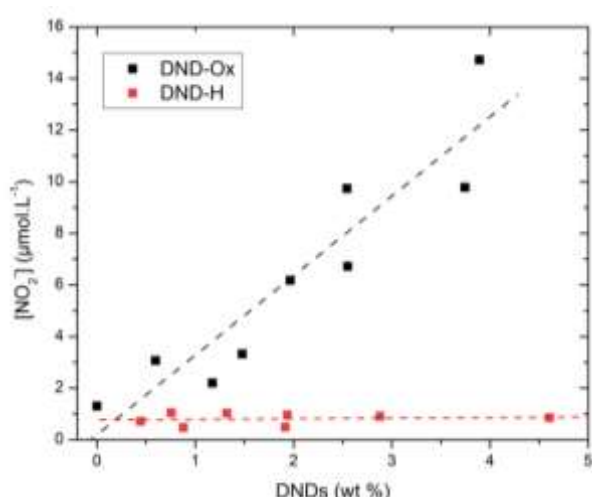
Figure 4 : Influence of the DNDs surface chemistry on the formation of nitrite ions during sonication.
