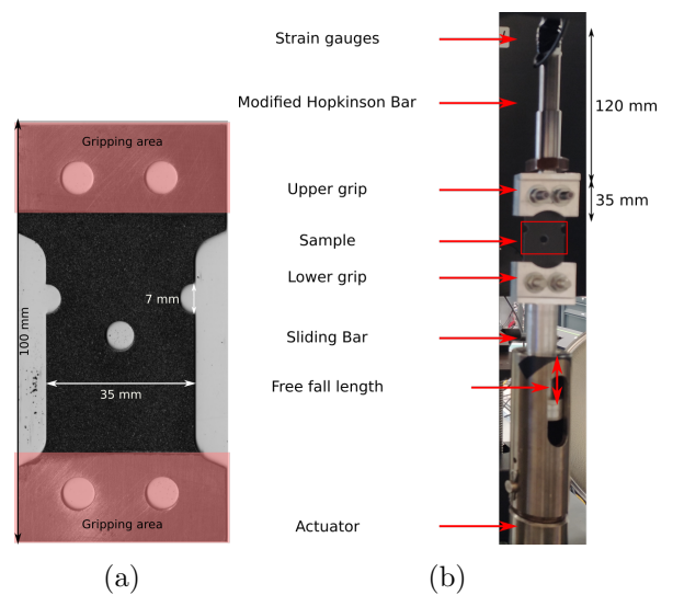
Figure 3: (a) Sample geometry and (b) Close-up view of the loading apparatus.
