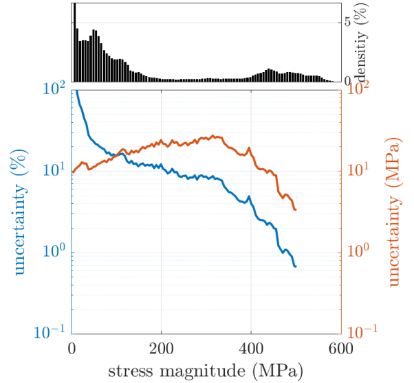
Figure 9: Stress uncertainty with respect to the stress magnitude. The stress magnitude occurrence in the test is given by the histogram while the blue and red lines are respectively the relative and absolute values of the stress uncertainty. The values are obtained after DDI post-treatment
