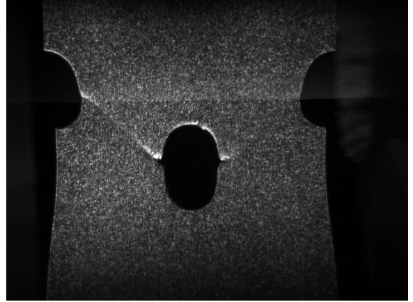
Figure 12: Last image (distortion-free) of the sample obtained during the test.
