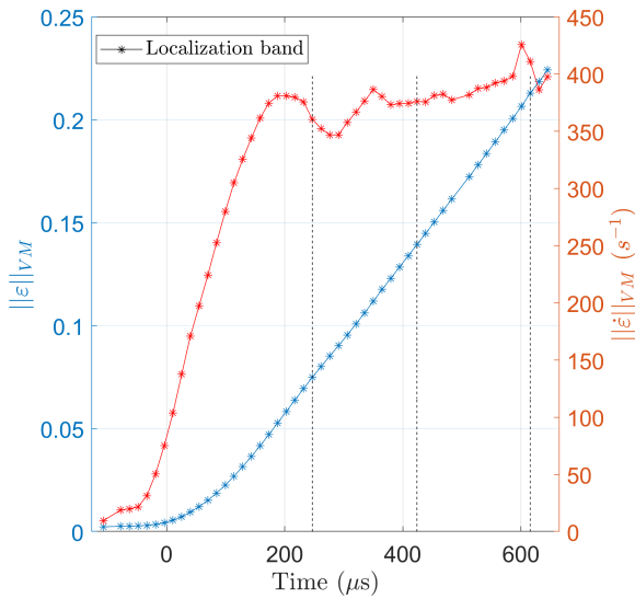
(a) Mean Von-Mises strains and strain-rates,
