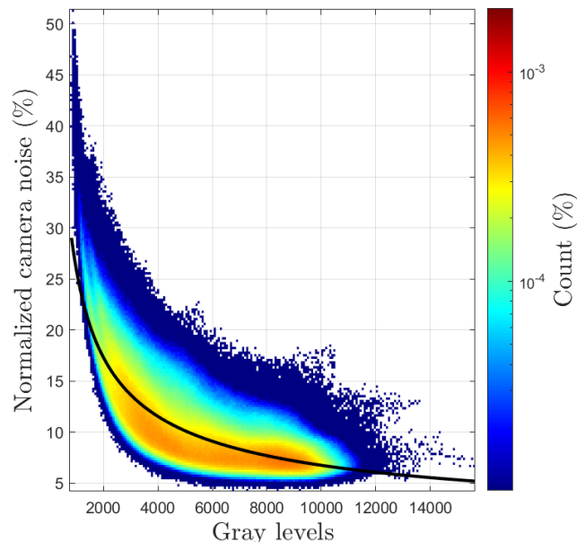
FIGURE 8 Normalized apparent camera noise (in %) versus the mean grey level. The colour denotes the pixel counts (in %), while the black line denotes the polynomials used to model the camera noise.
