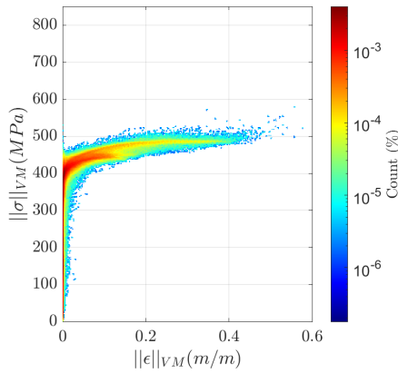
(b) Post-processed mechanical states,
