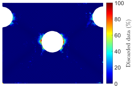
(c) Spatial localization of discarded states,
