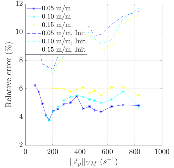
Figure 11: Relative stress identification error evolution with respect to the strain-rate. The stars represent the converged DDI solution while the dashed lines refer to the DDI initialization using set B parameters.
