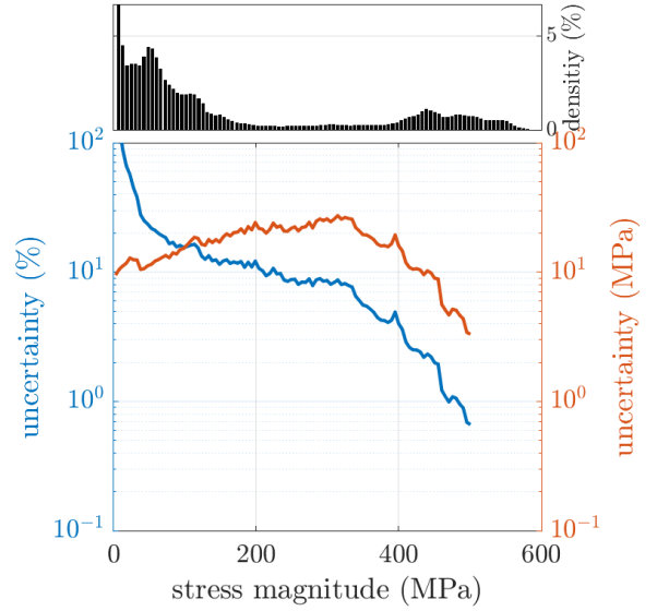
Figure 9: Stress uncertainty with respect to the stress magnitude. The stress magnitude occurrence in the test is given by the histogram while the blue and red lines are respectively the relative and absolute values of the stress uncertainty. The values are obtained after DDI post-treatment
