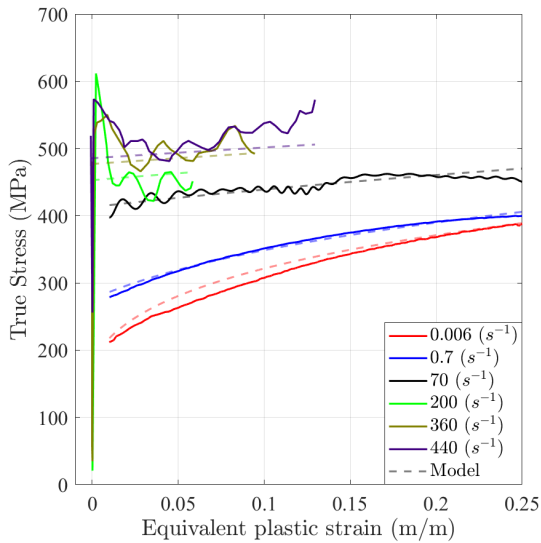
Figure 2: Modified Krupkowski model predictions (see Tab. 3) and tensile reference data reproduced, from [26] (from 0.006 to 70 s^{-1} using hydraulic test machines) and [24] (from 200 to 440 s^{-1} using dedicated non direct tensile loading on split Hopkinson bar apparatus).
