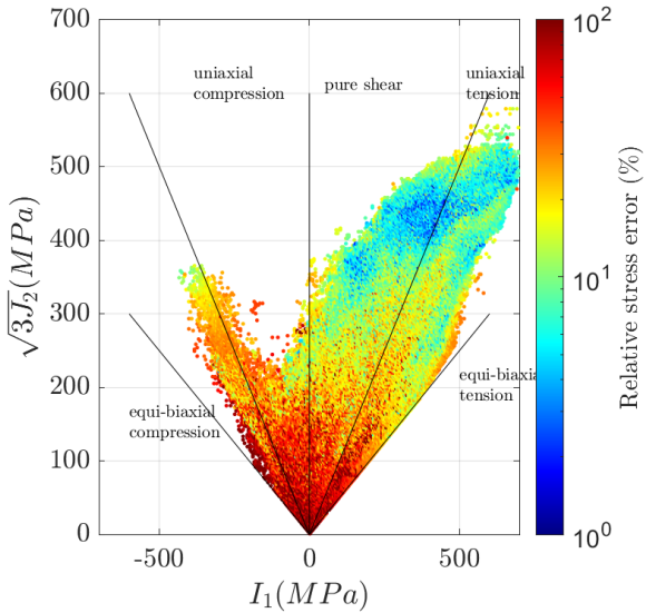
(b) Relative stress identification error,
