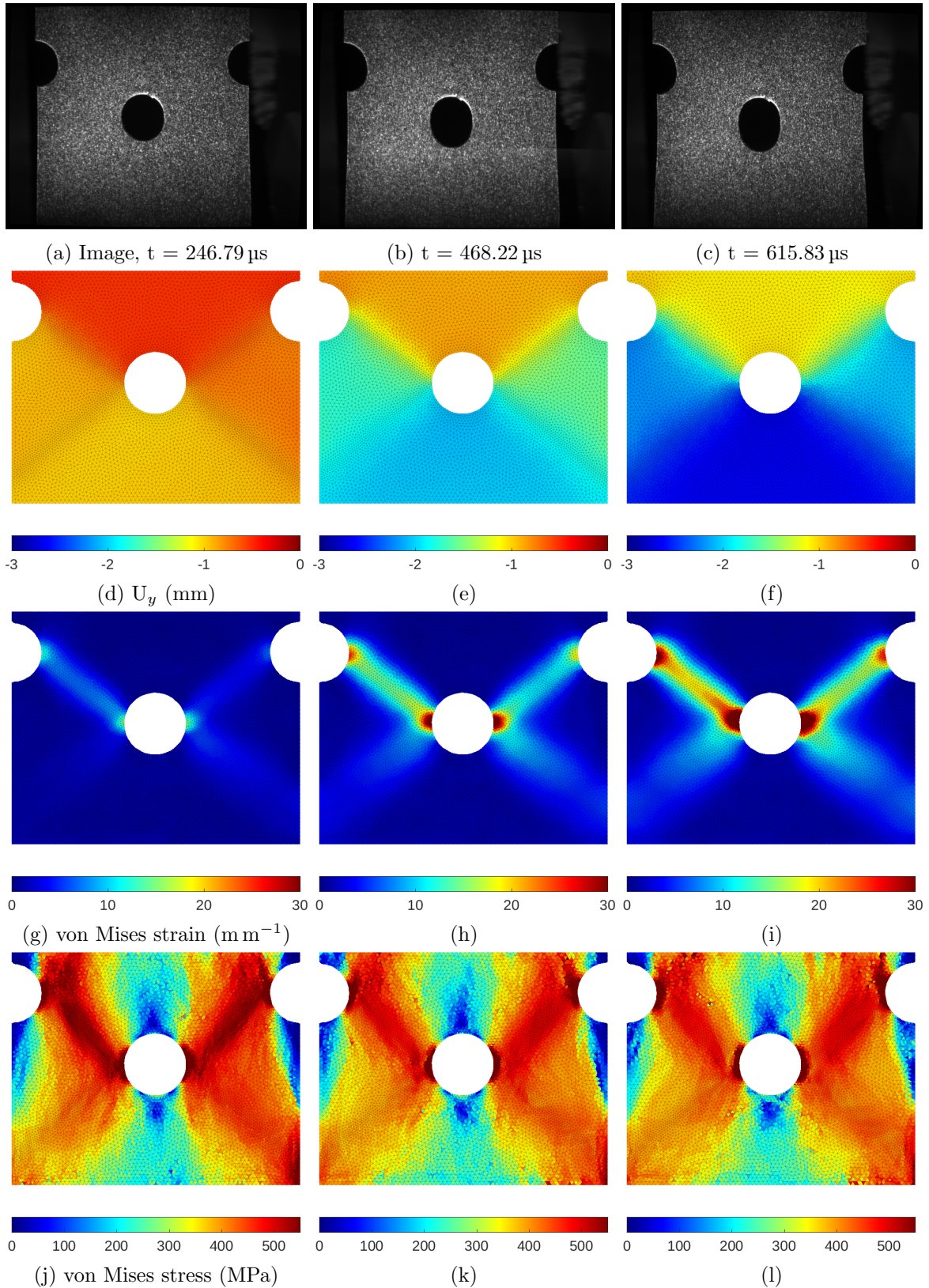
Figure 14: Distortion-free images (from a to c), axial displacement fields (from d to f), von Mises strain fields (from g to i) and von Mises stress fields (from j to l), extracted at 246.79, 468.22 and 615.83 \mu\text{s} during the dynamic tensile test.
