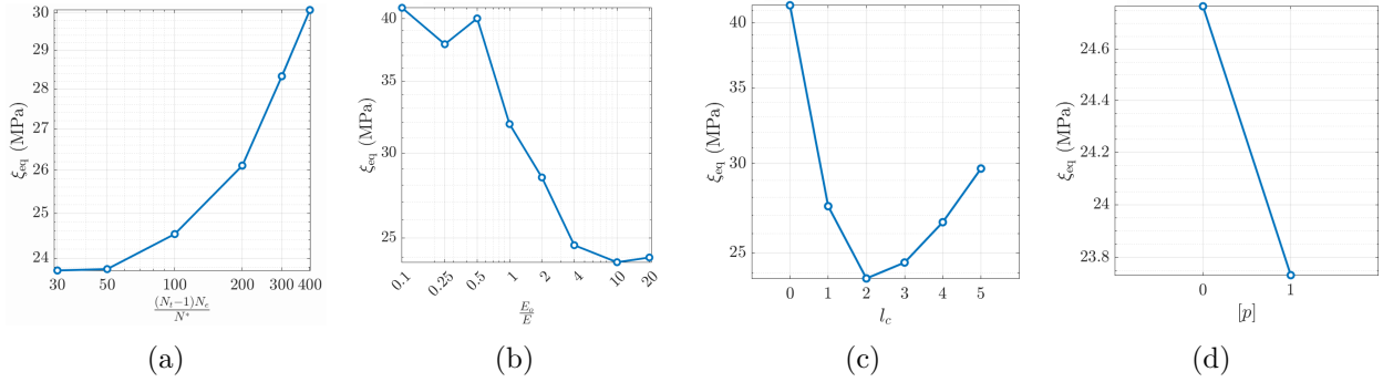
Figure 7: Evolution of \xi_{eq} with respect to the DDI parameters \mathbf{P} = \{[p], l_c, \frac{E_0}{E}, \frac{(N_t-1)N_e}{N^*}\} . 3 over 4 parameters are fixed: (a) \mathbf{P} = \{1, 2, 10, -\} , (b) \{1, 2, -, 30\} , (c) \{1, -, 10, 30\} and (d) \{-, 2, 10, 30\} . Note that the y-scale differs from one figure to another.
