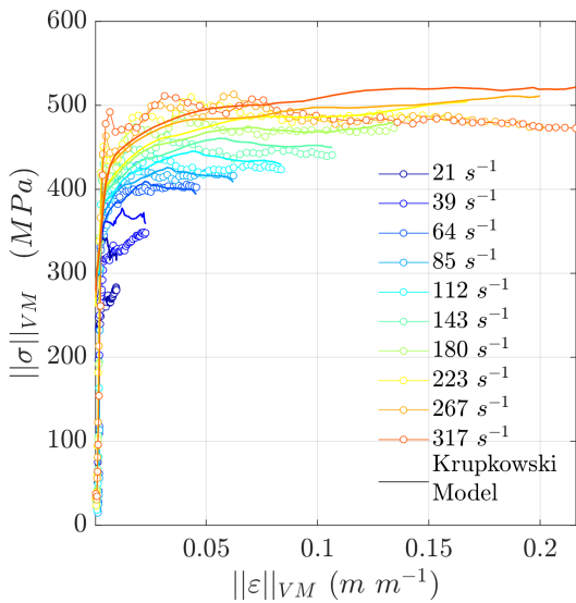
(a) Mean experimental stress-strain responses and model predictions,
