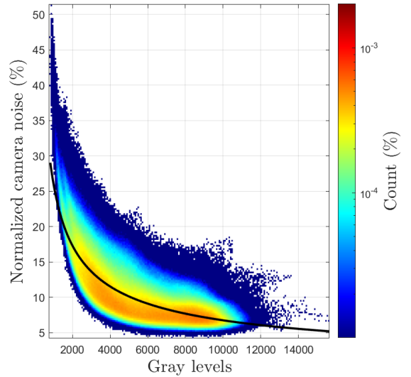
Figure 5: Normalized apparent camera noise (in %) versus the mean grey level. The colour denotes the pixel counts (in %), while the black line denotes the polynomials used to model the camera noise.
