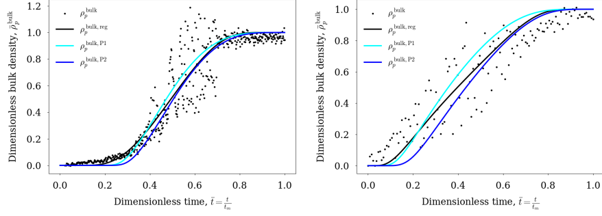
(a) TUDA - Run27 (light aggregate).
