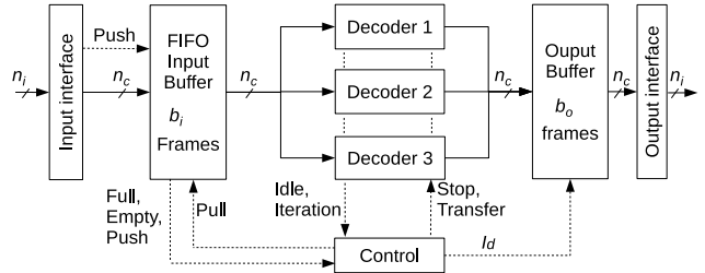
Fig. 1. Multi-core architecture.
