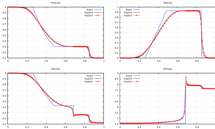
FIGURE 1. Sod shock tube for Euler equations. The CFL are CFL_{\text{explicit}} = 0.4 and CFL_{\text{implicit}} = 0.4 .
