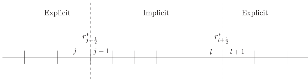
FIGURE 8. Example of a mesh divided into several subdomains.
