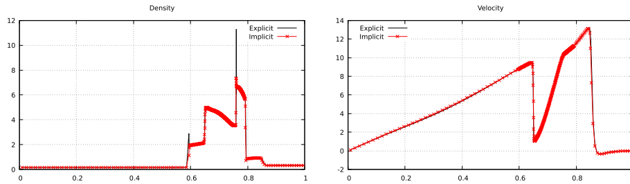
FIGURE 6. Blast waves for Euler equations. The CFL is CFL = 0.4 .
