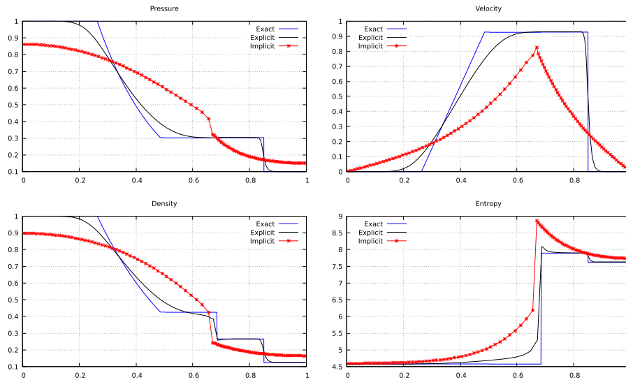
FIGURE 4. Sod shock tube for Euler equations. The CFL are CFL_{\text{explicit}} = 0.4 and CFL_{\text{implicit}} = 537 (only one time step).
