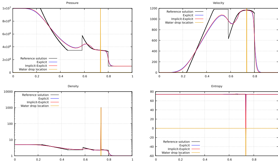
FIGURE 10. Sod shock tube perturbed by a water drop.
