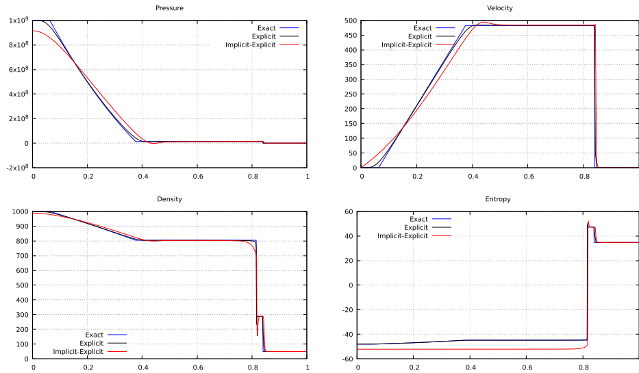
FIGURE 9. Two-phase shock tube for Euler equations.
