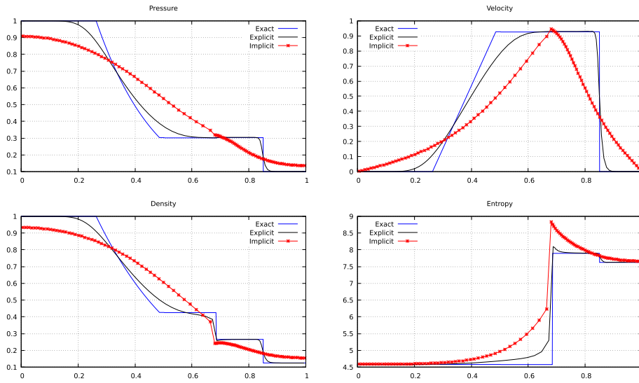
FIGURE 3. Sod shock tube for Euler equations. The CFL are CFL_{\text{explicit}} = 0.4 and CFL_{\text{implicit}} = 80 .
