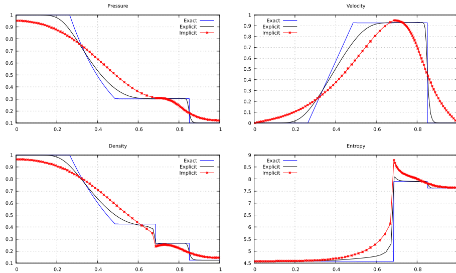
FIGURE 2. Sod shock tube for Euler equations. The CFL are CFL_{\text{explicit}} = 0.4 and CFL_{\text{implicit}} = 40 .
