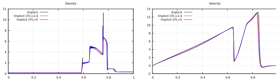
FIGURE 7. Blast waves for Euler equations. Comparison between the explicit acoustic solver scheme and the implicit scheme with multiple CFL.
