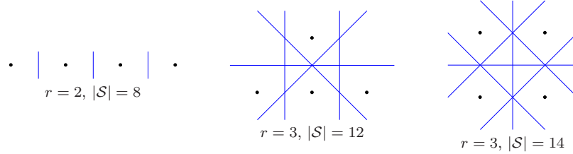
Fig. 3.1 Linearly separable bipartitions of a set of p = 4 points \bar{v}_i in \mathbb{R}^2 (the dots in the figure). Possible separating hyperplanes are the drawn lines. We have not represented any separating line associated with the partition (\emptyset, [1 : p]) or ([1 : p], \emptyset) , so that |\mathcal{S}| = 2(n_s + 1) , where n_s is the number of represented separating lines. We have set r := \dim(\text{vect}\{\bar{v}_1, \dots, \bar{v}_p\}) + 1 .
