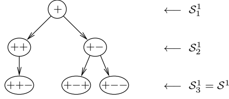
Fig. 5.1 Half of the \mathcal{S} -tree for example 3.2 (the other half is obtained by swapping the '+'s and the '-'s). Top-down arrows indicate descent; the sign sets \mathcal{S}_k^1 are defined by (5.1).
