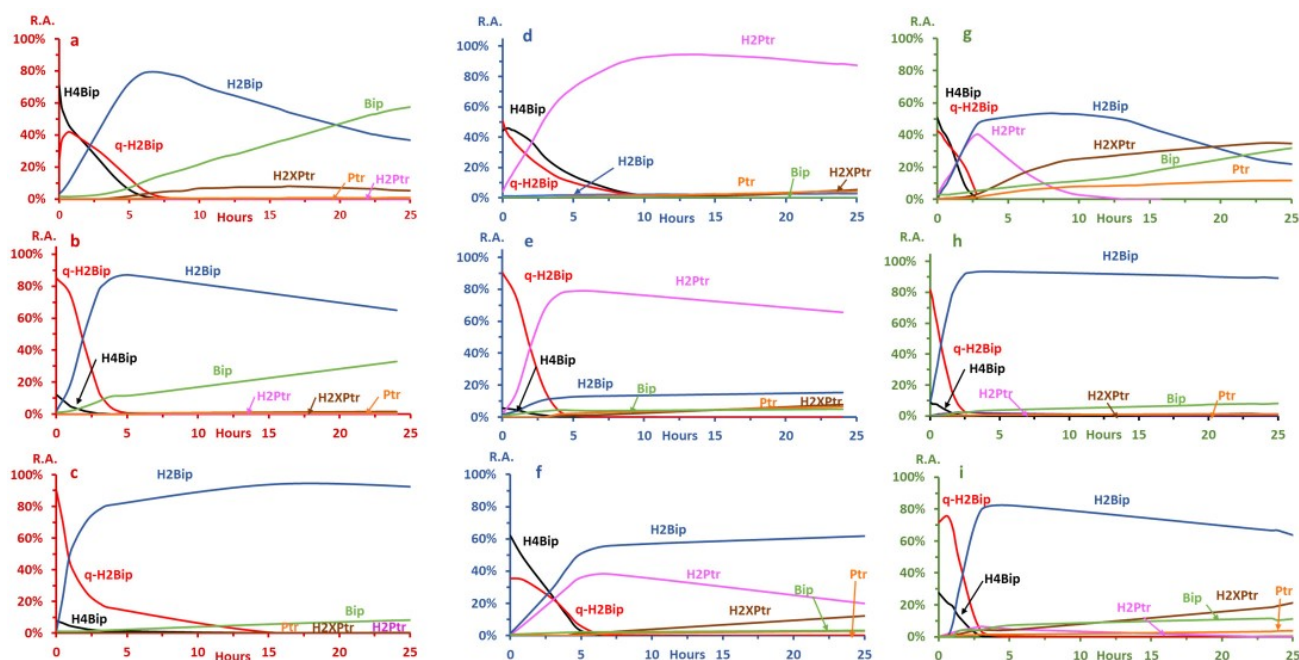
Figure 3. H4Bip autoxidation kinetics as a function of pH and type of buffer (0.1 M ammonium buffer): (a–c) \text{pH} \leq 3.0 ; (d–f) \text{pH} 7.4 ; and (g–i) \text{pH} 5.4 . (a) \text{pH} 2.8 , formate; (b) \text{pH} 3.0 , acetate; (c) \text{pH} 2.8 , citrate; (d) \text{pH} 7.4 , formate; (e) \text{pH} 7.4 , acetate; (f) \text{pH} 7.4 , citrate; (g) \text{pH} 5.4 , formate; (h) \text{pH} 5.4 , acetate; and (i) \text{pH} 5.4 , citrate. R.A.—Relative abundance. R.A. is expressed as the percentage of each peak-area ratio (PAR) (PAR—peak area of the considered product/IS peak area) relative to the total sum of all PARs.
