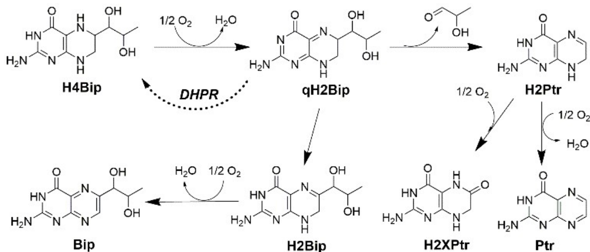
Figure 1. Autoxidation pathways of tetrahydrobiopterin (H4Bip) according to Refs. [2,18–23]. qH2Bip—quinonoid dihydrobiopterin; H2Bip—7,8-dihydro-biopterin; H2Ptr—dihydro-pterin; H2XPtr—dihydro-xanthopterin; Bip—biopterin; Ptr—pterin; DHPR—dihydro-pteridine reductase.
