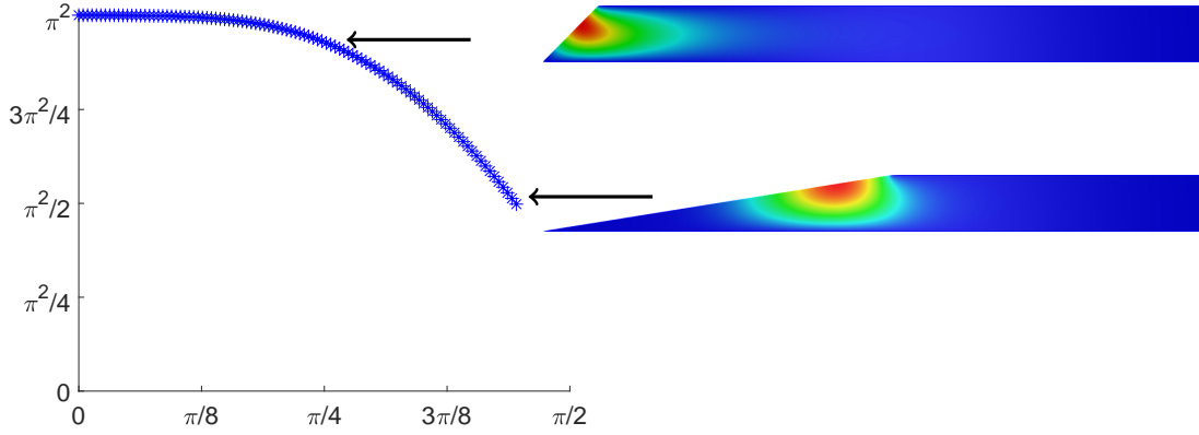
Figure 8: Curve \alpha_1 \mapsto \mu_1^{\alpha_1} for \alpha_1 \in (0, 9\pi/20) . According to Theorem 2.1, this gives the bound \lambda_{\dagger}^{\kappa} of the essential spectrum of A^{\kappa} . The two pictures correspond to eigenfunctions associated with \mu_1^{\alpha_1} for \alpha_1 = \pi/4 and \alpha_1 = 9\pi/20 .
