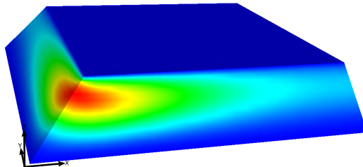
Figure 11: Eigenfunction associated with the first eigenvalue of \sigma_d(A^{\kappa}) for \kappa = (1, 1) . We find \lambda_1^{\kappa} \approx 0.90\pi^2 .
