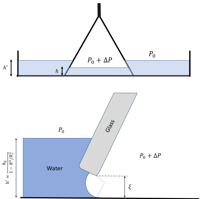
FIG. 3. Three-step route to levitation. Upper panel: During the first stage the pressure increase expels the inner water film through the cracks between the bottom edge of the funnel and the crystallizer. The increased inner-volume mitigates the pressure excess and prevents lift-off. Lower panel (close-up): When the water is fully expelled, the glass takes off but air is still trapped inside by a capillary bridge connecting the glass to the bottom of the crystallizer. The bridge ruptures when the geometric constraint \xi \leq 2r is no longer met.
