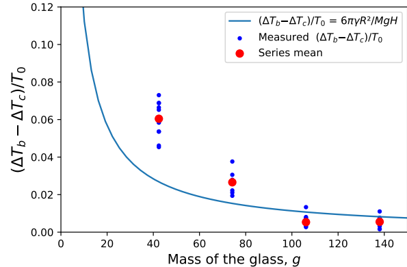
FIG. 5. Evolution of the critical temperature vs glass mass and height of the water layer. The solid line corresponds to the capillary bridge stability condition 15
