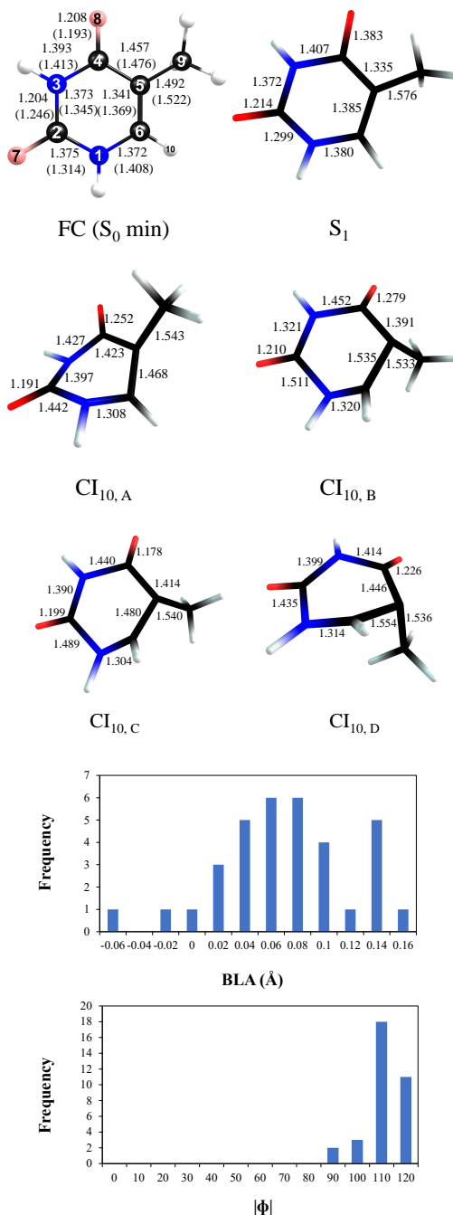
Figure 4: FC ( S_{0, \text{min}} ) is optimized geometry of ground state in gas-phase with atom numbering and crystallographic data 57 given in parenthesis, while S_1 is the last snapshot that remains in S_1 state. All CI_{10} corresponds to the structures at the hopping point. The (BLA/Å, \phi /°) values are; S_1 (0.167, 20.53), CI_{10,A} (0.055, -100.57), CI_{10,B} (0.134, 110.07), CI_{10,C} (0.033, 102.06), CI_{10,D} (0.062, 109.41). \phi is defined as the H_{10}C_6C_5C_9 dihedral angle. The histograms of BLA and \phi of geometries at 34 hopping points are also presented.
