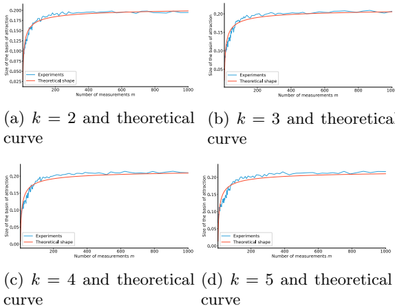
Fig. 5: Size of the basin of attraction with respect to the number of measurements m with different number of spikes k . The theoretical curve is obtained by a least squares fitting of the function C_1\sqrt{1 - C_2/\sqrt{m}} parametrized by C_1 and C_2 .
