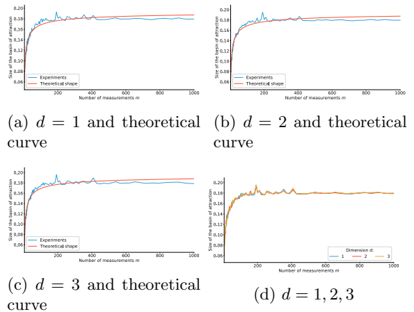
Fig. 4: Size of the basin of attraction with respect to the number of measurements m with various dimensions d . The theoretical curve is obtained by a least squares fitting of the function C_1 \sqrt{1 - C_2/\sqrt{m}} parametrized by C_1 and C_2 .
