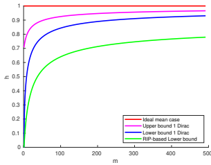
Fig. 2: A schematic representation of the shape of the curves obtained by our theorems for \lambda = 1 . Red: h = 1 (exact bound mean case), Magenta: h = \sqrt{1 - 1.5/\sqrt{m}} (one spike upper bound), Blue: h = \sqrt{1 - 3/\sqrt{m}} (one spike lower bound), Green: h = 0.9 \cdot (1 - 3/\sqrt{m}) (ideal RIP-based lower bound). The chosen constants are for illustration purpose only and are not originated from our Theorems. True sizes of basins of attraction are investigated experimentally in the next Section.
