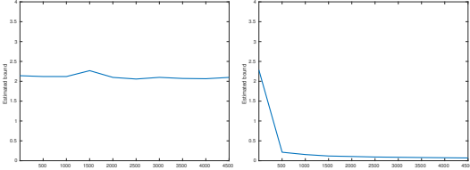
Fig. 8: Evaluation of \|A\partial_u^2\phi(\theta)\|_2 for k = 1 and different d . Left: c(\omega) = 1 . Right: c(\omega) = 1/(1 + \lambda^2 \|\omega\|_2^2/d) . We observe that \|A\partial_u^2\phi(\theta)\|_2 can be bounded independently of d .
