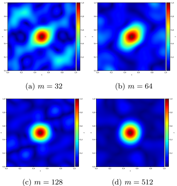
Fig. 3: Back-projection of the signal x_0 = \delta_t observed with m random Fourier measurements. We observe that the measurement operator converges to a Gaussian kernel as m increases.
