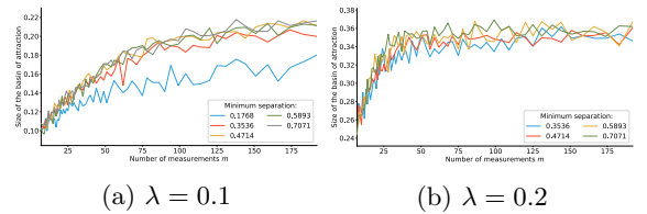
Fig. 6: Size of the basin of attraction with respect to the minimum separation \epsilon .
