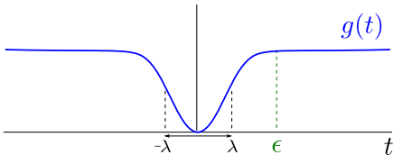
Fig. 1: A representation of g(t) = 2(1 - e^{-\frac{t^2}{2\lambda^2}}) for the case of one Dirac measure. The parameter \lambda is generally chosen so that it is a multiple of \epsilon . The function is convex on [-\lambda, \lambda] .
