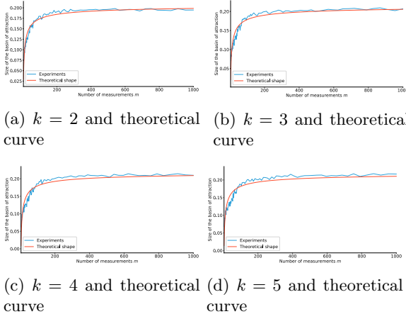
Fig. 5: Size of the basin of attraction with respect to the number of measurements m with different number of spikes k . The theoretical curve is obtain by a least squares fitting of the function C_1\sqrt{1 - C_2/\sqrt{m}} parametrized by C_1 and C_2 .
