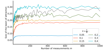
Fig. 7: Size of the basin of attraction with respect to the choice of the resolution parameter \lambda . Minimum separation is \epsilon = 0.5 .
