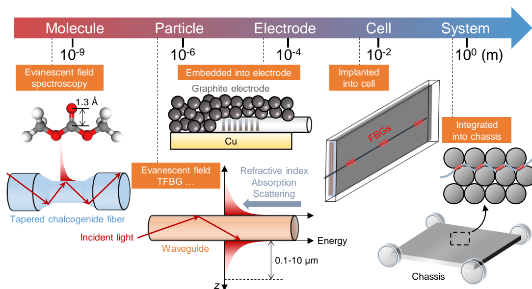
Figure 5 | Monitoring of batteries by fiber optic sensor at different length scales.
