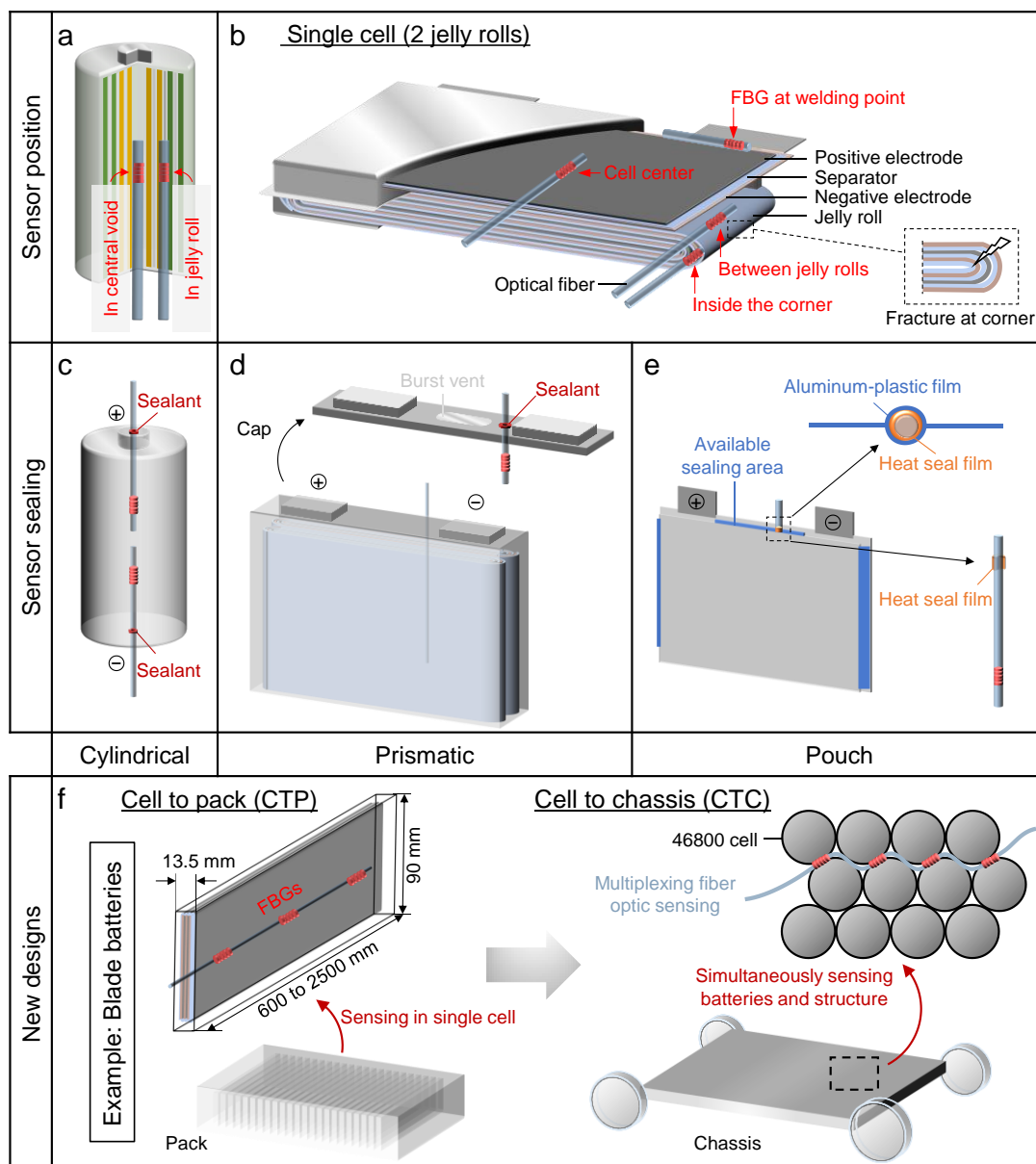
Figure 4 | Implanting fiber optic sensors. a,b, Sensor positions in cylindrical (a) and flat jelly rolls (b, taking a single cell with two jelly rolls as an example) for the pouch and prismatic cells. c-e, Sensor sealing in cylindrical (c), prismatic (d), and pouch (e) cells. f, Integrating optical sensor with new engineering designs, including cell to pack (CTP, left) and cell to chassis (CTC, right).
