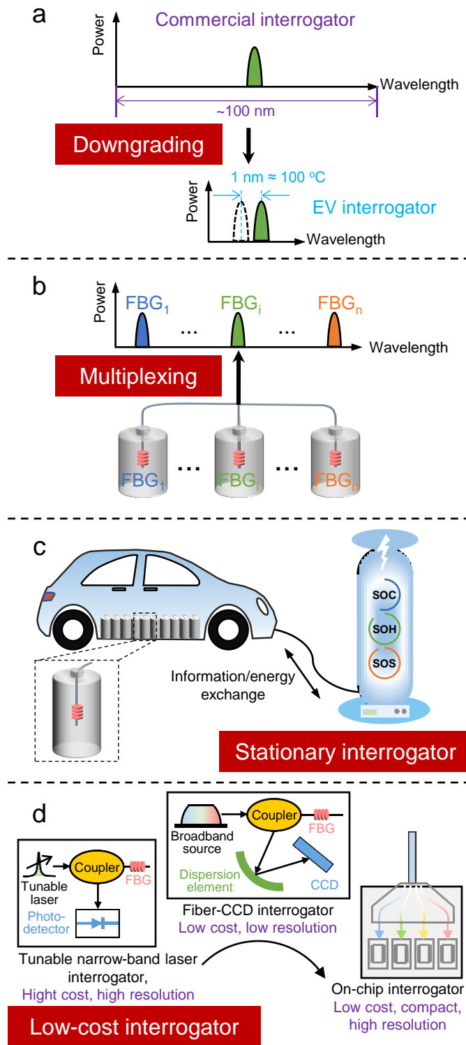
Figure 3 | Reducing the cost of interrogation. a, Downgrading the wavelength range of interrogator. b, Wavelength division multiplexing of multiple optical sensors in a single interrogation channel. c, Stationary interrogator for sharing the interrogation cost. d, Low-cost interrogators by fiber-CCD interrogator 36 and on-chip interrogator 37 .
