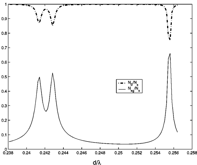
FIG. 7. Decomposition of the scattering field on resonant and evanescent modes for an incident Gaussian beam focused on the center of the crystal (see arrow 1 in Fig. 6).
