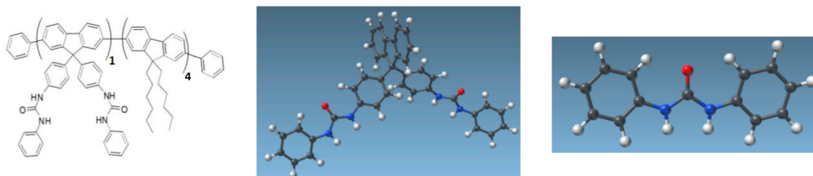
Figure 3. (Left): Chemical structure of FF-UR polymer. Adapted from [39], with the permission of AIP Publishing. (Middle): Fluorene monomer carrying two urea-based sensing moieties (SAMSON software). Reproduced from [40], with the permission of John Wiley and Sons. (Right): focus on the sensing moieties (SAMSON software). Atom color code: black for carbon, white for hydrogen, blue for nitrogen, red for oxygen. Reproduced from [40], with the permission of John Wiley and Sons.
