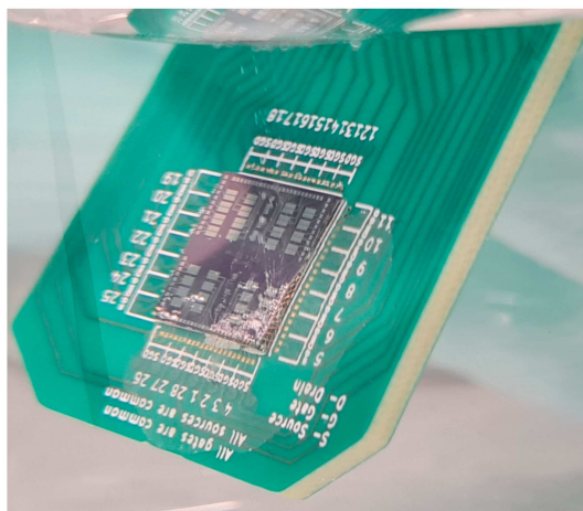
Figure A2. Bubble formation (bottom right corner of the chip) in water along the contacts when applying voltage larger than 1 V, due to water electrolysis.
