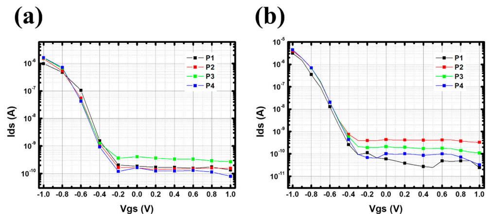
Figure A4. Logarithmic I–V transfer curve of p-CNTFETs in pH 7 phosphate buffer solution (PBS) after (a) two months and (b) three months. All transistors were 5\ \mu\text{m} channel devices. V_{ds} was set to +0.8\ \text{V} and V_{gs} was swept from -1\ \text{V} to +1\ \text{V} .
