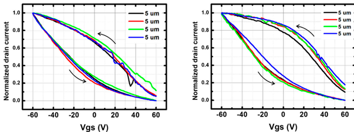
Figure 5. Normalized I–V transfer curves (current level divided by I_{on} ) of 5 \mu\text{m} channel ( left ) p-CNTFETs and ( right ) f-CNTFETs at drain–source voltage ( V_{ds} ) of +5 V in air. Four different 5 \mu\text{m} transistors are shown for each type of FETs. The arrows indicate gate–source voltage ( V_{gs} ) sweeping direction.
