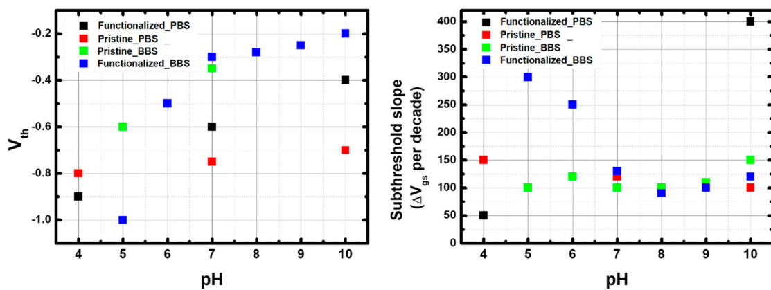
Figure 12. (left) V_{th} and (right) Subthreshold slope of p-CNTFETs and f-CNTFETs in different buffer solutions.
