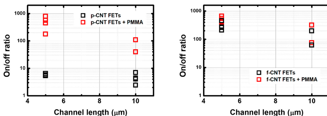
Figure 4. I_{on}/I_{off} ratio of (left) p-CNTFETs and (right) f-CNTFETs before and after PMMA passivation with channel length of 5 \mu m and 10 \mu m.
