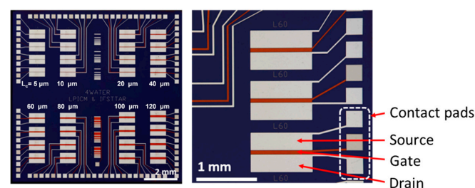
Figure 2. Pre-fabricated chip ( 10 \text{ mm} by 10 \text{ mm} ) with gate, source and drain electrodes and contact pads for wire-bonding. Channel length L_c varies from 5 \mu\text{m} to 120 \mu\text{m} .
