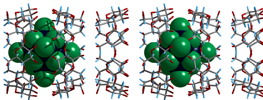
Figure 3. Selected fragment of the crystal structure of Mo_6Cl_{14}@2CD \cdot CD . Mo—dark blue, Cl—green, O—red, C—gray, H—light blue. Disordering of the cluster is omitted for clarity.
