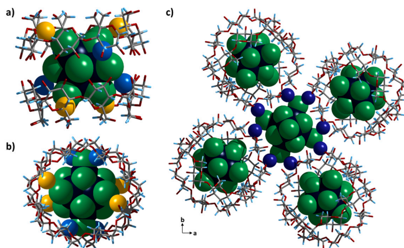
Figure 2. Selected fragments of crystal structure of W_6Cl_{14}@2CD \cdot 0.5W_6Cl_{14} . Side (a) and top (b) view of inclusion compound \{[W_6Cl^I_8Cl^a_6]@(\gamma-CD)_2\}^{2-} . Highlight of the packing involving CD-free clusters and its four neighboring moieties. (c). W—dark blue, Cl—green, O—red, C—gray, H—light blue, H3, H5 and H4 involved in hydrogen bonding—space-filling blue, orange and indigo, respectively.
