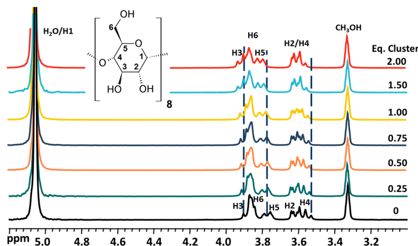
Figure 4. ^1H NMR spectra from the titration of 2 mM \gamma -CD solution with the Mo_6Cl_{14} in D_2O/CD_3OD (50/50 vol.%) mixture with 5 vol.% of DCl_{conc} .
