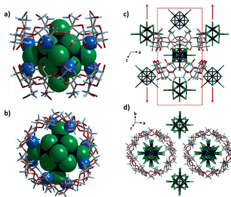
Figure 1. Selected fragments of crystal structure of \text{Mo}_6\text{Cl}_{14}\text{@}2\text{CD}\cdot 2\text{Mo}_6\text{Cl}_{14} . Side (a) and top (b) view of inclusion compound \{[\text{Mo}_6\text{Cl}_8\text{Cl}^{\text{a}}_6]\text{@}(\gamma\text{-CD})_2\}^{2-} . Highlight showing the close environment of the CD-free clusters: side (c) and top (d) view. Color code: Mo—dark blue, Cl—green, O—red, C—gray, H—light blue, H involved in hydrogen bonding—space-filling blue, \text{Mo}_6\text{-CD@Mo}_6\text{@CD-Mo}_6 complex—red frame. Red arrows indicate growing directions of omitted \text{Mo}_6\text{-CD@Mo}_6\text{@CD-Mo}_6 complex. Disordering of cluster is omitted for clarity in pictures (a,b).
