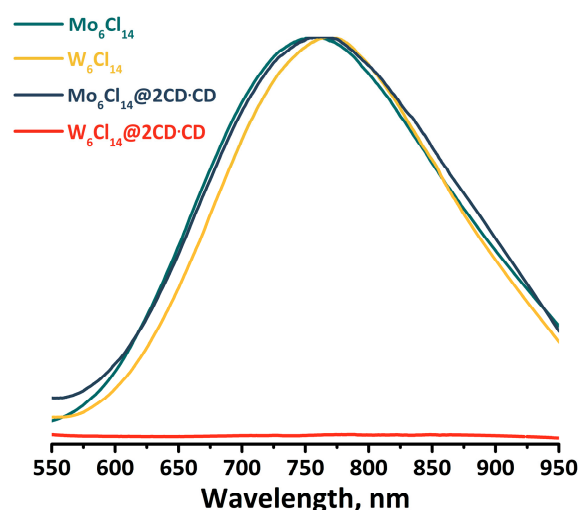
Figure 5. Normalized and smoothed emission spectra of compounds in solid state.
