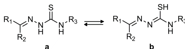
Scheme 1 Tautomeric forms of thiosemicarbazone ligands
