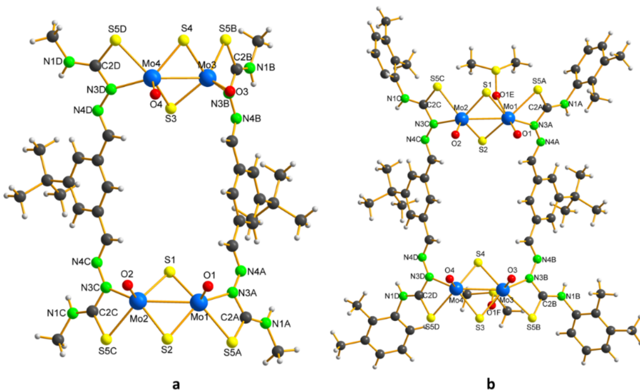
Figure 4. Molecular structure of [(\text{Mo}_2\text{O}_2\text{S}_2)_2(\text{L}^4)_2] : a) in front and b) lateral views. Colour code: Mo (blue), C (gray), O (red), N (green), and S (yellow).
