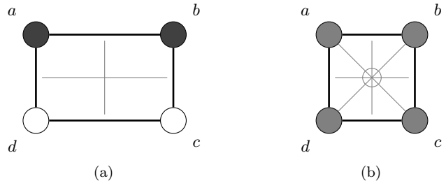
FIG. 1. Geometric representation of the permutation symmetries of U_{abcd} . The vertices are labelled clockwise with the orbital indices a, b, c and d . (a) The complex conjugation of non-real orbitals is graphically represented as a transformation of black vertices into white ones (and vice versa). The permutations form the group m'm2' which describes the symmetries of a rectangle with 2 white and 2 black vertices. (b) The permutations of real orbitals form the group D_4 which describes the symmetries of a square.
