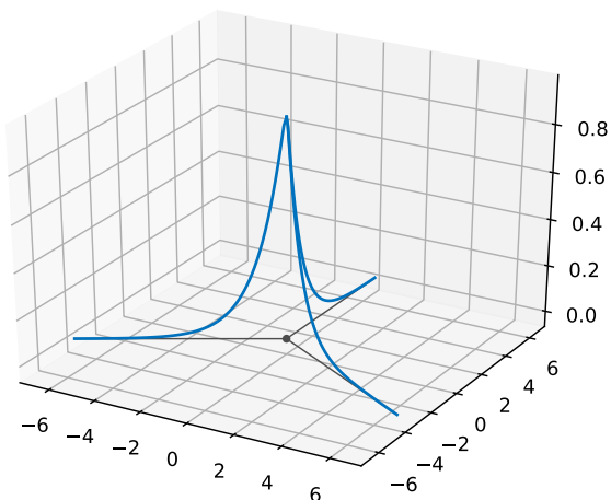
FIGURE 2. The function Q_\beta on a 3-star graph for \beta = -5/2
