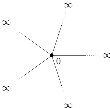
FIGURE 1. A star graph with 5 edges.
