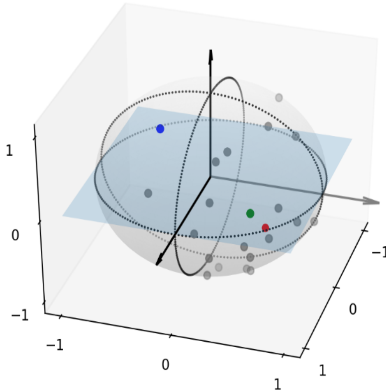
Figure 3: Example of representation on the Poincare sphere: In gray, the N individual different Stokes vectors of the time-series; Red Point: Stokes vector of the main eigenvector, Blue Point: Stokes vector of the second eigenvector, Green point: Stokes vector for the whole time-series
