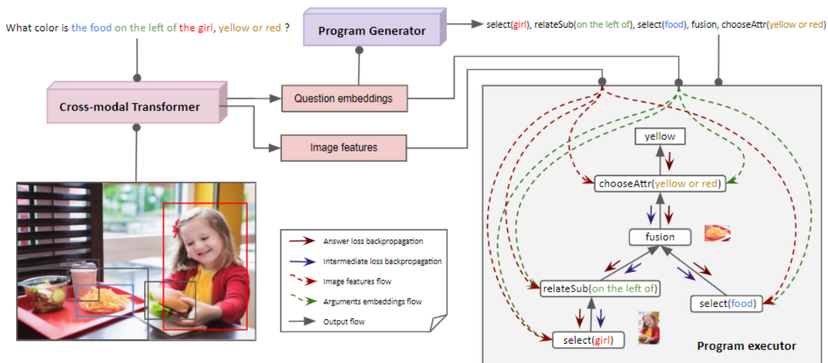
Figure 1: The proposed modular VQA framework: The (question, image) pair is used by a transformer model to generate aligned cross-modal embeddings for words and objects. These are used by a Program Generator module to produce a program (represented as a sequence of sub-task modules), which will be then applied by the Program Executor module to the image to answer the question. The proposed work focuses on improving the Program Executor by using several curriculum learning (CL) strategies.
