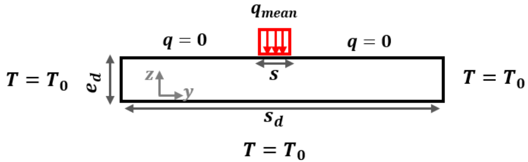
Figure 4: 2D liner thermal model
