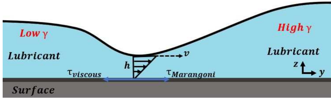
Figure 5: Thermal Marangoni model
