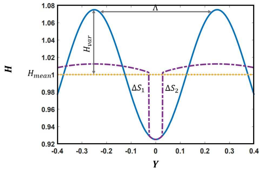
Figure 17: Lubricant distribution before and after the ring passage
