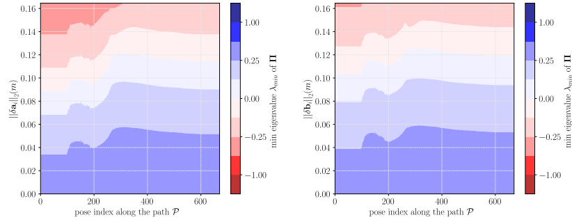
(a) Stability versus the norm of the exit point error \delta \mathbf{a}_i . (b) Stability of the robot versus the norm of the anchor point error \delta \mathbf{b}_i .
