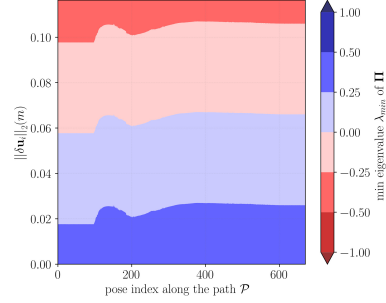
Fig. 6: Stability of the robot along \mathcal{P} versus the norm of the sensor position error
