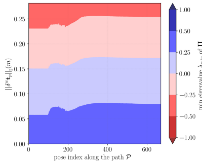
Fig. 5: Stability of the robot along \mathcal{P} versus the position estimation error \delta^w \mathbf{t}_p
