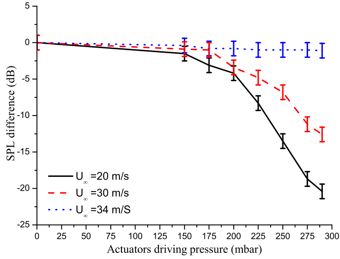
Figure 17: Evolution of the fundamental frequency SPL (dB) against the actuators driving pressure for different velocities.
