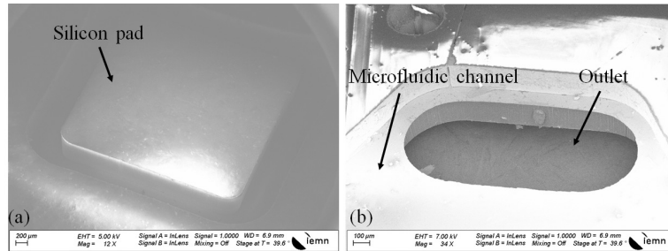
Figure 5: SEM (Scanning Electron Microscopy) pictures of the MMMS microvalve: (a) the membrane and the silicon pad (b) the extremity of the microfluidic channel with the outlet
